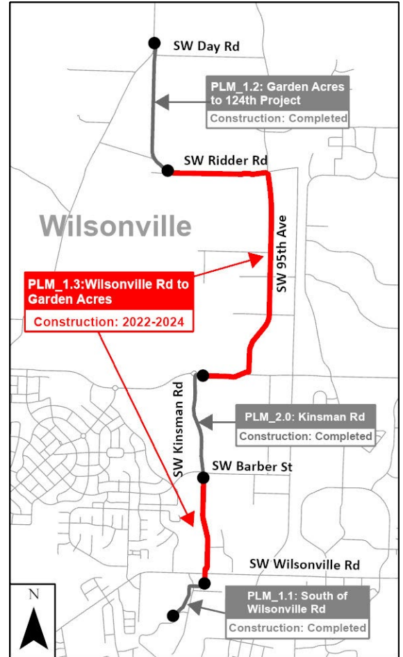
Map of PLM 1.3 pipeline construction area.
