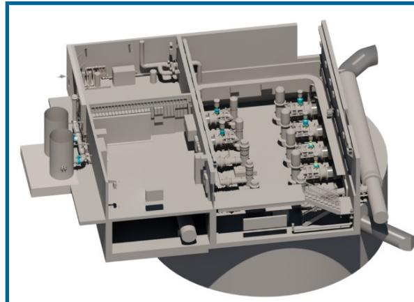
Raw Water Pump Station and Caisson
