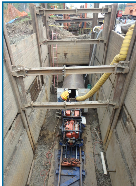
Installation of 78-inch steel casing at Kinsman Road Partnership Project
